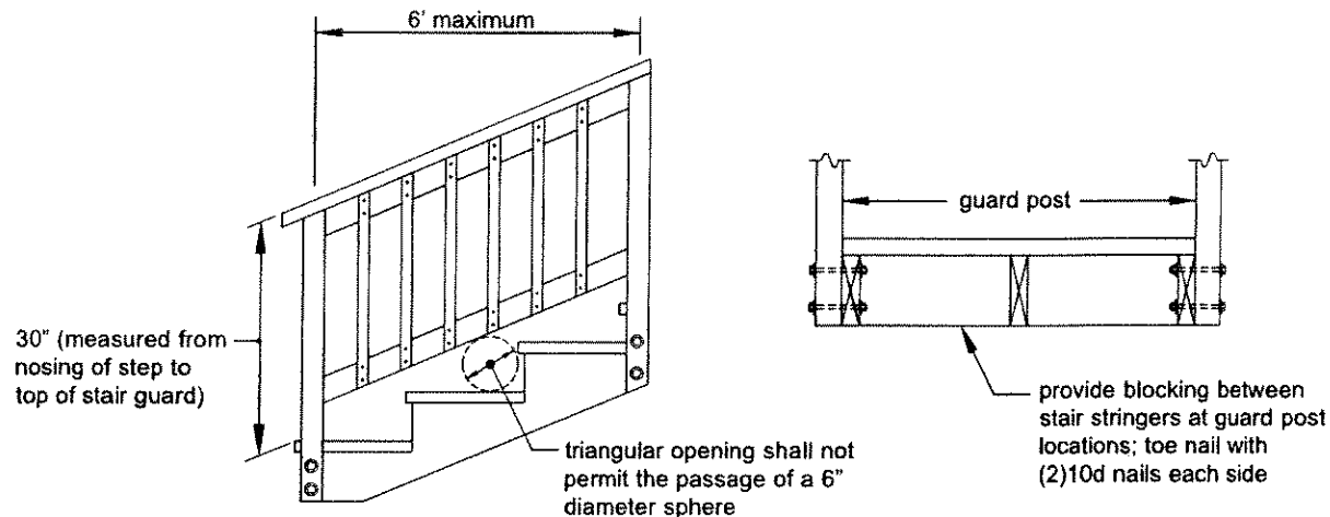
Figure 32 STAIR GUARDS
