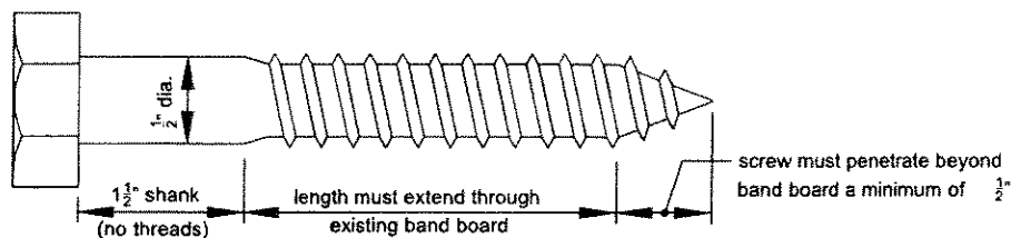
Figure 16 LAG SCREW
