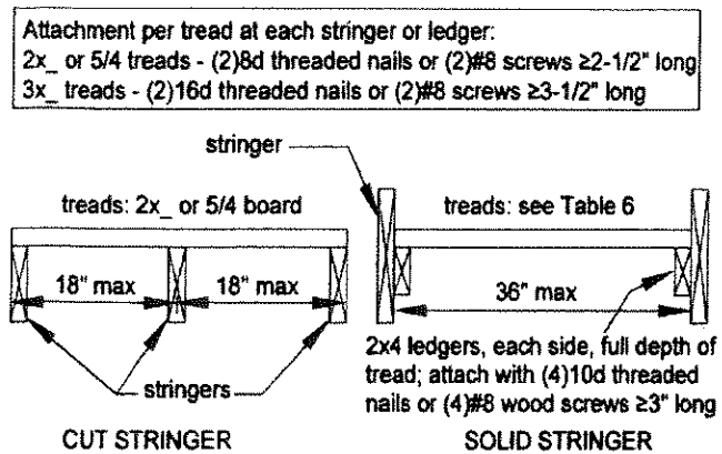
Figure 31 STAIRWAY TREADS
