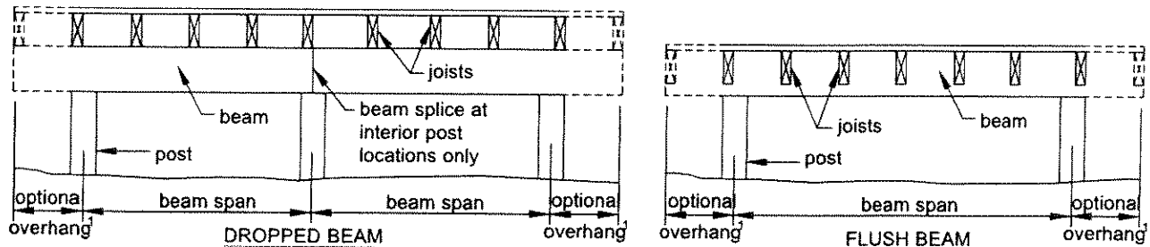
Figure 3 BEAM TYPES
