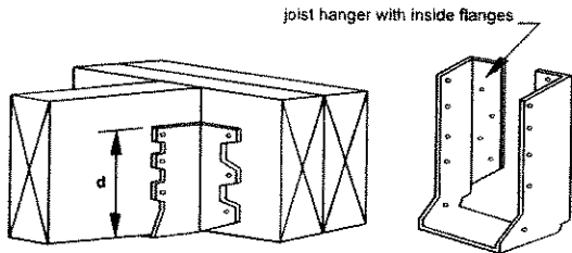
Figure 9 JOIST HANGERS
