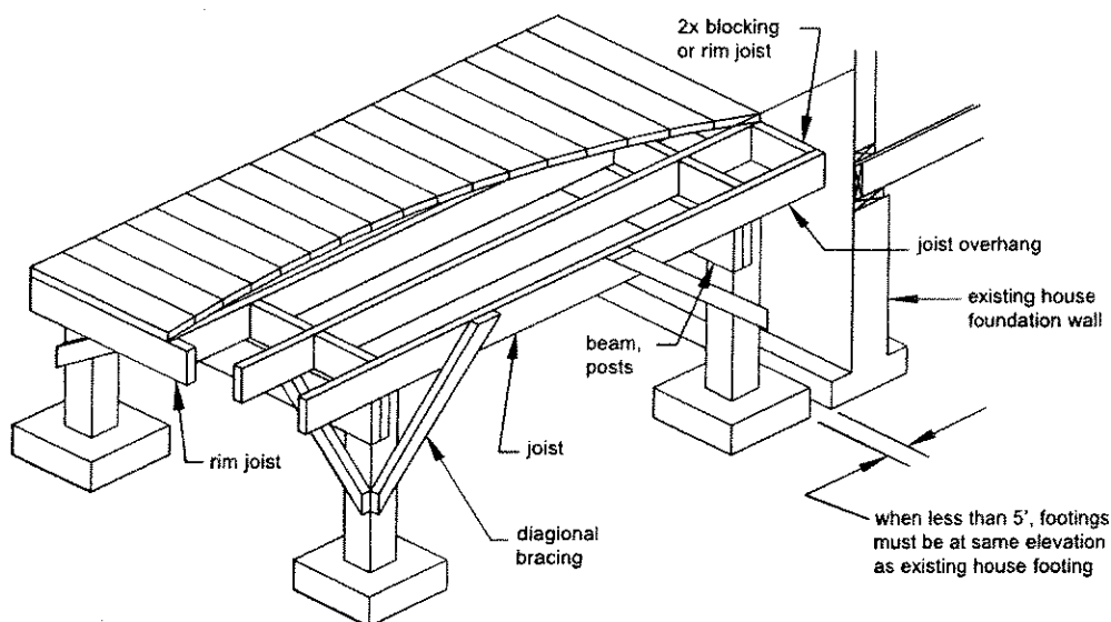
Figure 17 FREE-STANDING DECK
