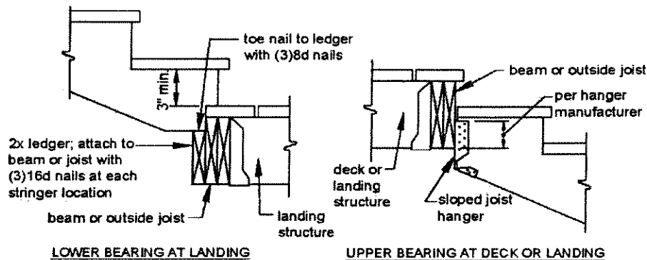
Figure 28 STRINGER BEARING
